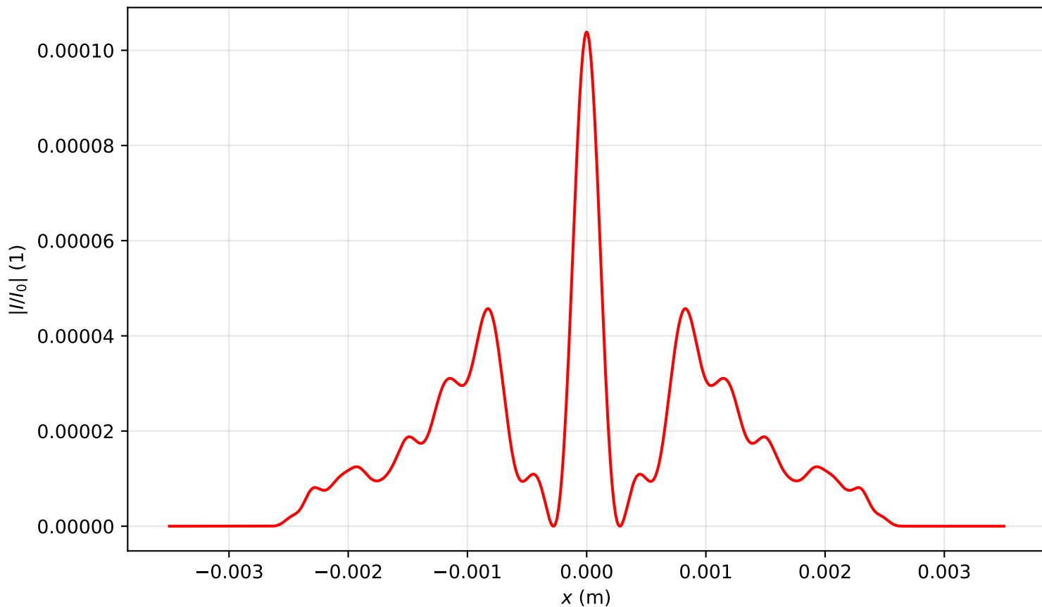
Intensity profile I(x, y = 0, z = 1.831)/I_0 , P_{in}=6.0P_{cr} , artificial time
